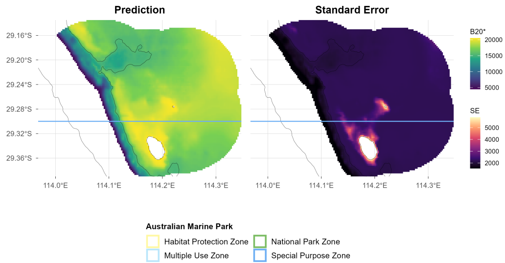
Figure 11.3: Demersal fish - Large Reef Fish Index*: spatial plots of distribution probability and uncertainty from stereo-BRUV groundtruthing. Commonwealth marine park boundaries are shown.
