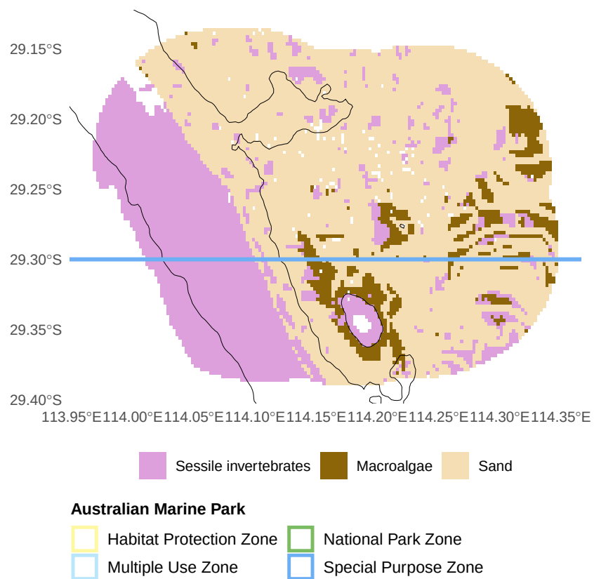
Figure 3: Predicted benthic distribution probability from stereo-BRUV groundtruthing. Commonwealth marine park boundaries are shown.
