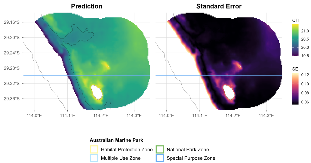
Figure 12.3: Demersal fish - Reef Fish Thermal Index: spatial plots of distribution probability and uncertainty from stereo-BRUV groundtruthing. Commonwealth marine park boundaries are shown.
