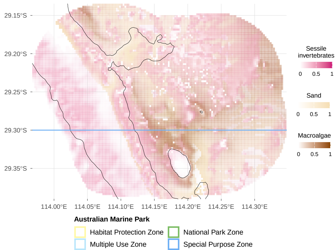
Figure 2: Predicted dominant benthic type from stereo-BRUV groundtruthing. Commonwealth marine park boundaries are shown.
