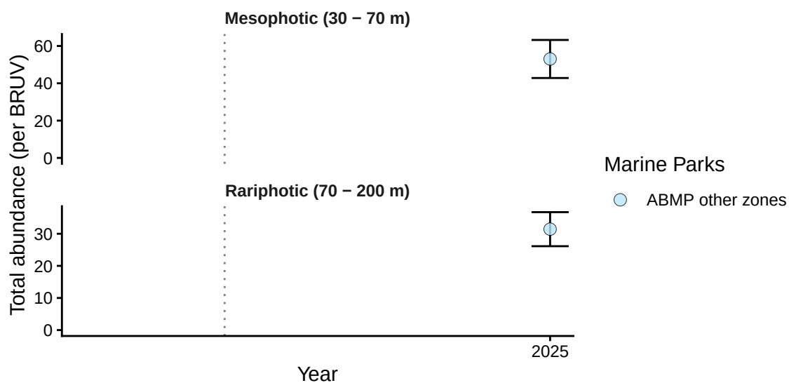
Figure 10.1: Demersal fish - Total abundance: benchmark plot by depth contour from stereo-BRUV groundtruthing. ABMP = Abrolhos Marine Park (Commonwealth). All deployments fall within the Special Purpose Zone, so no zone contrast is shown.
