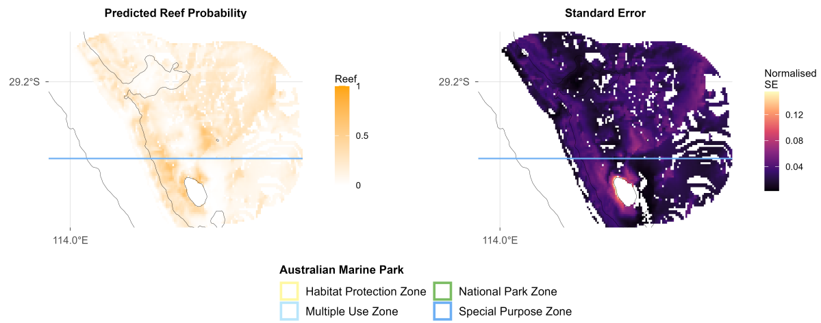
Figure 4: Predicted reef distribution probability and uncertainty from stereo-BRUV groundtruthing. Commonwealth marine park boundaries are shown.
