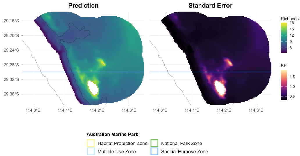
Figure 9.3: Demersal fish - Species richness: spatial plots of distribution probability and uncertainty from stereo-BRUV groundtruthing. Commonwealth marine park boundaries are shown.
